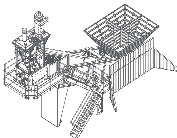
JUMPER 1500/2500
